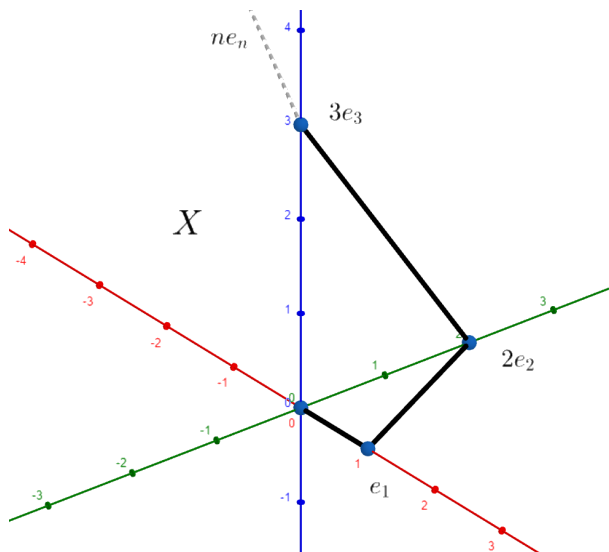
FIGURE 1. Representation of the space (inside \ell^1 )
